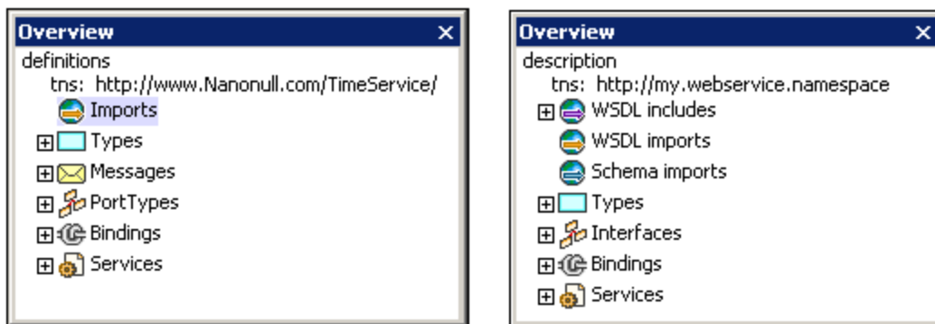
Overview entry helper in WSDL 1.1 (left) and WSDL 2.0 (right).
